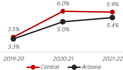
Dropout Rate
